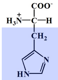
Histidine
