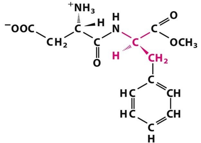
L-Aspartyl-D-phenylalanine methyl ester (bitter)
