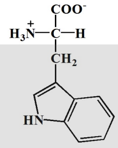
Tryptophan
