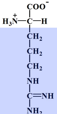
Arginine
