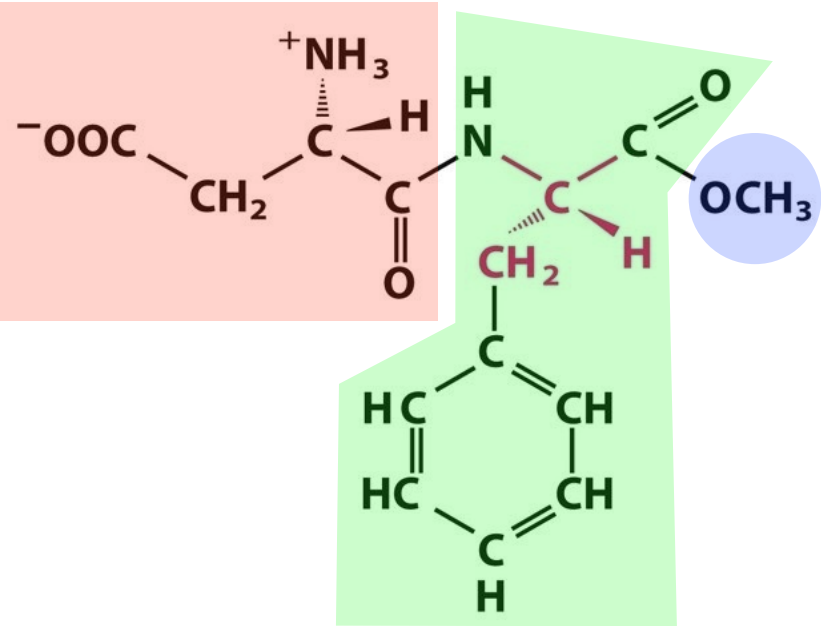
L-Aspartyl-L-phenylalanine methyl ester (aspartame) (sweet)
