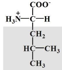
Leucine
