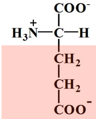
Glutamate
