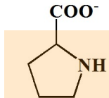
Proline
