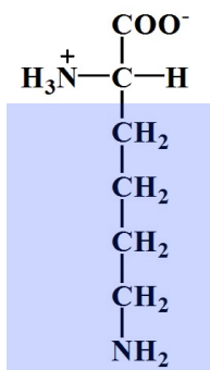
Lysine
