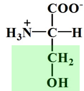
Serine
