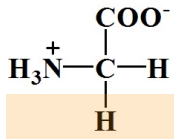
Glycine
