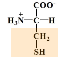
Cysteine
