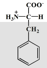
Phenylalanine
