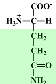
Glutamine
